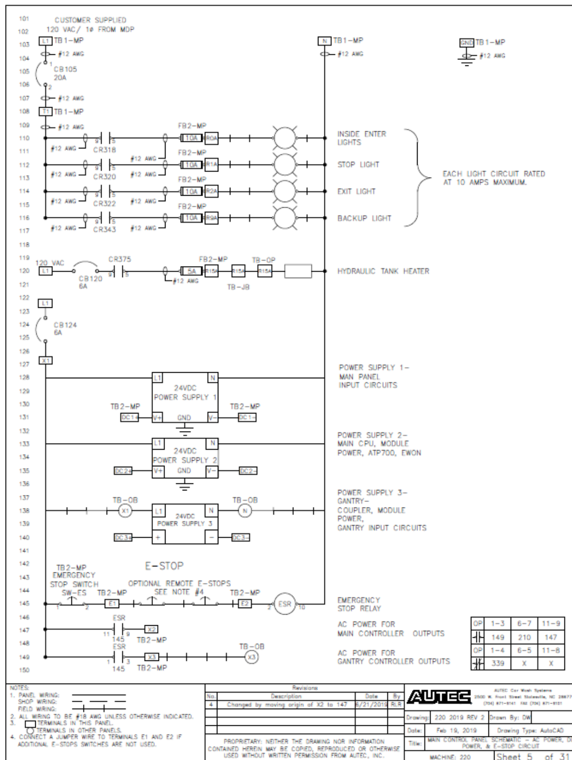
Fig 9-5 Main Control Panel – AC & DC Power, Emergency Stop
