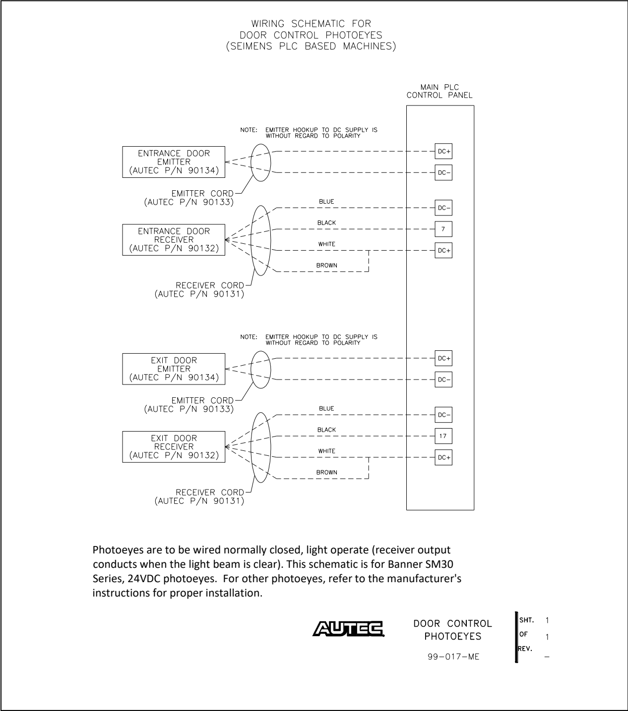
Fig 13-1 Door Control Photoeye Wiring
