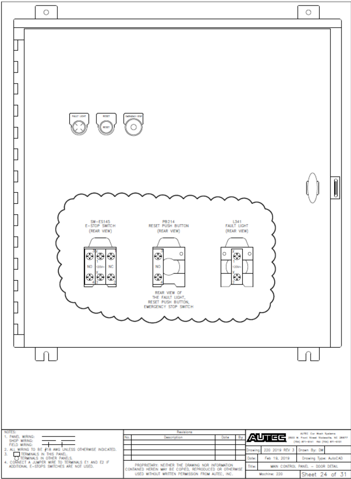
Fig 9-24 Main Control Enclosure – Door Detail
