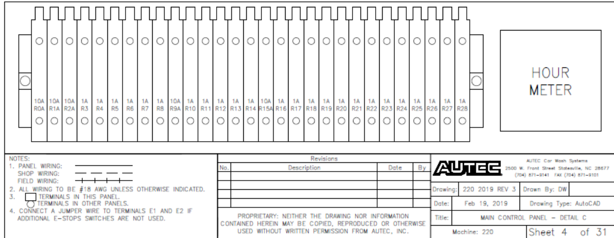
Fig 9-4 Main Control Panel – Detail C
