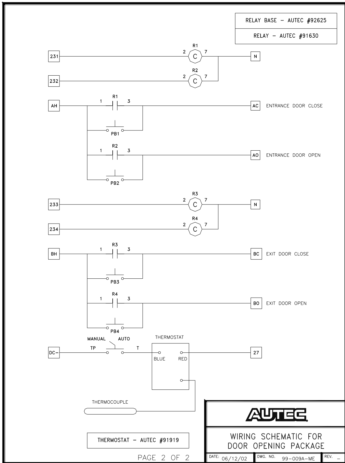
Fig 13-3 Wiring Schematic for Optional Door Control Package
