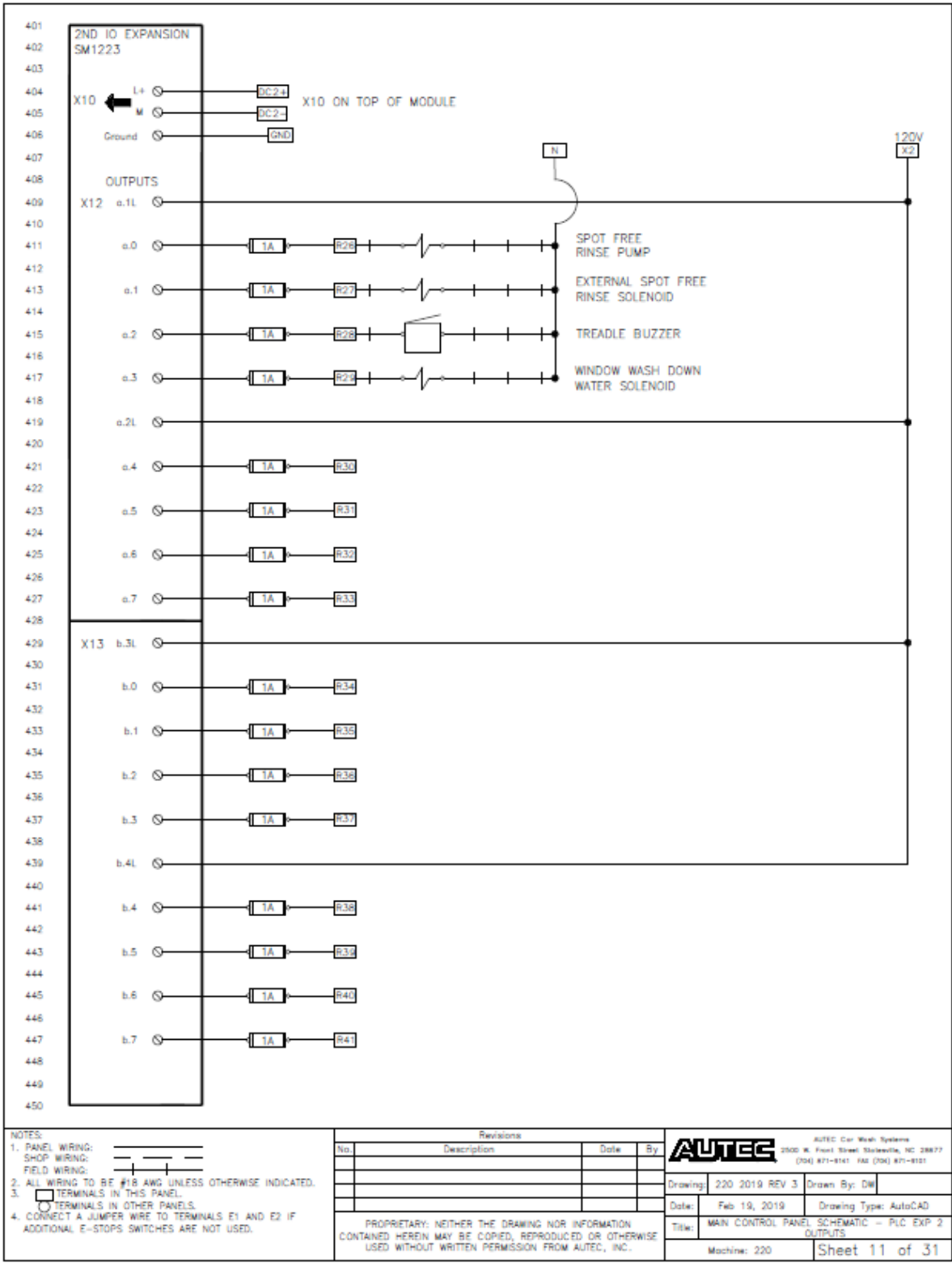
Fig 9-11 Main Control Panel – PLC Module 2 Outputs
