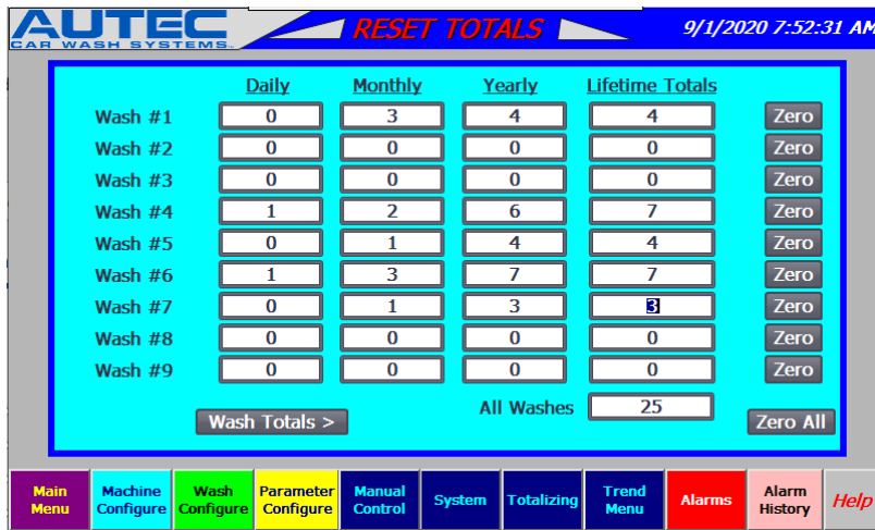
Figure 7-42 Reset Totals Screen
