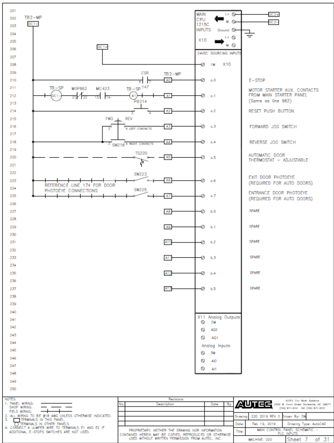
Fig 9-7 Main Control Panel – PLC Main Inputs
