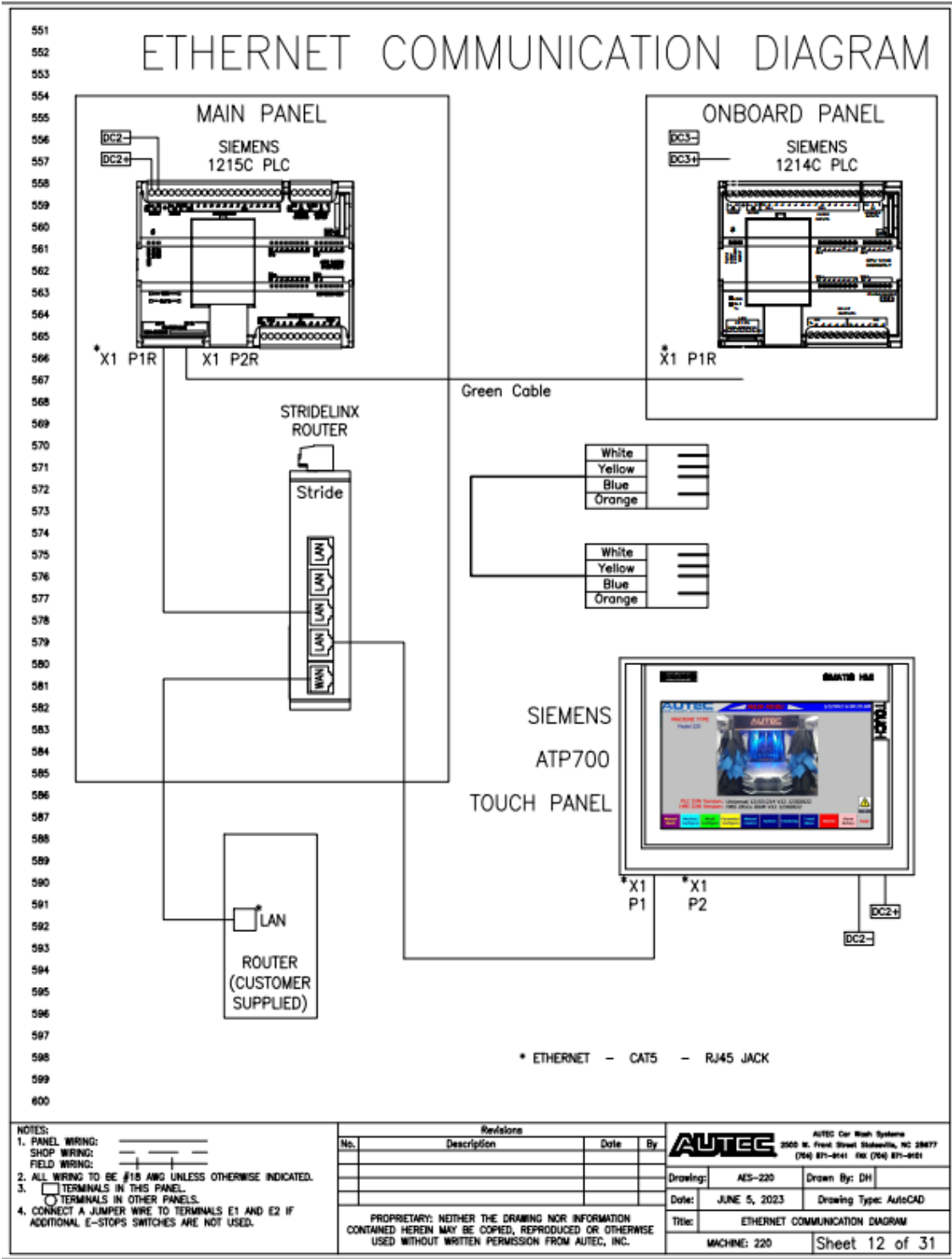
Fig 9-12 Ethernet Communications Diagram
