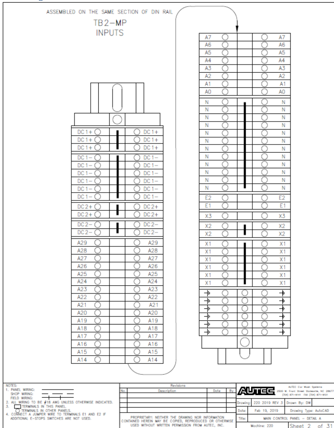
Fig 9-2 Main Control Panel – Detail A
