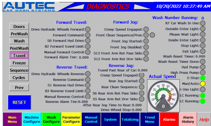
Figure 7-33 Travel Screen
