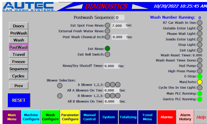
Figure 7-32 Postwash Screen
