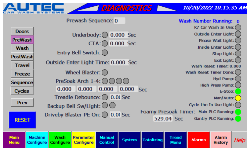
Figure 7-30 Prewash Screen
