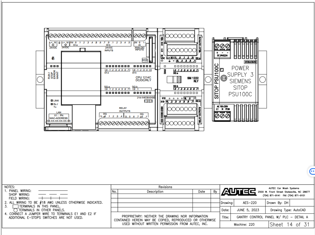
Fig 9-14 Gantry Control Panel –Detail A
