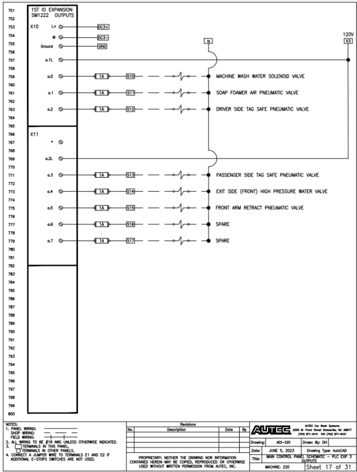
Fig 9-17 Gantry Control Panel – Outputs #2
