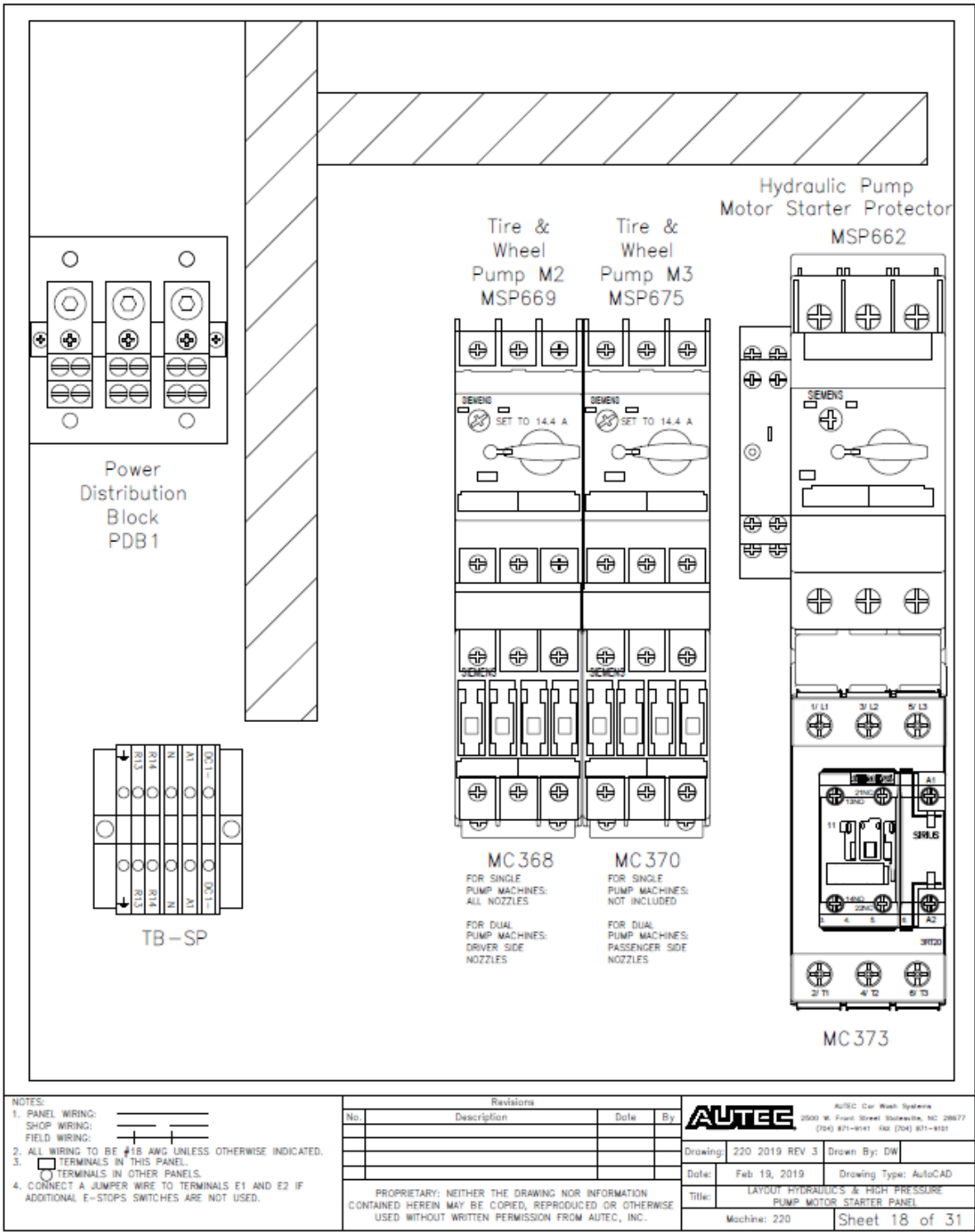
Fig 9-18 Hydraulic & High Pressure Pump Motor Starters
