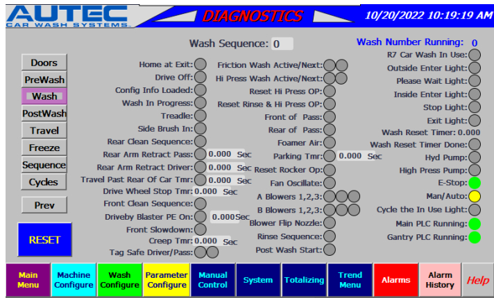
Figure 7-31 Wash Screen
