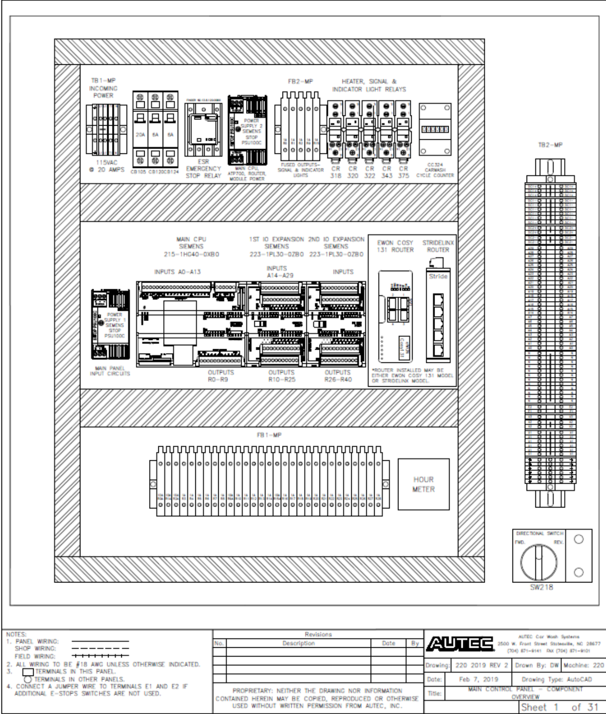
Fig 9-1 Layout Main Panel Backplane Devices
