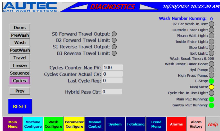
Figure 7-36 Cycles Screen
