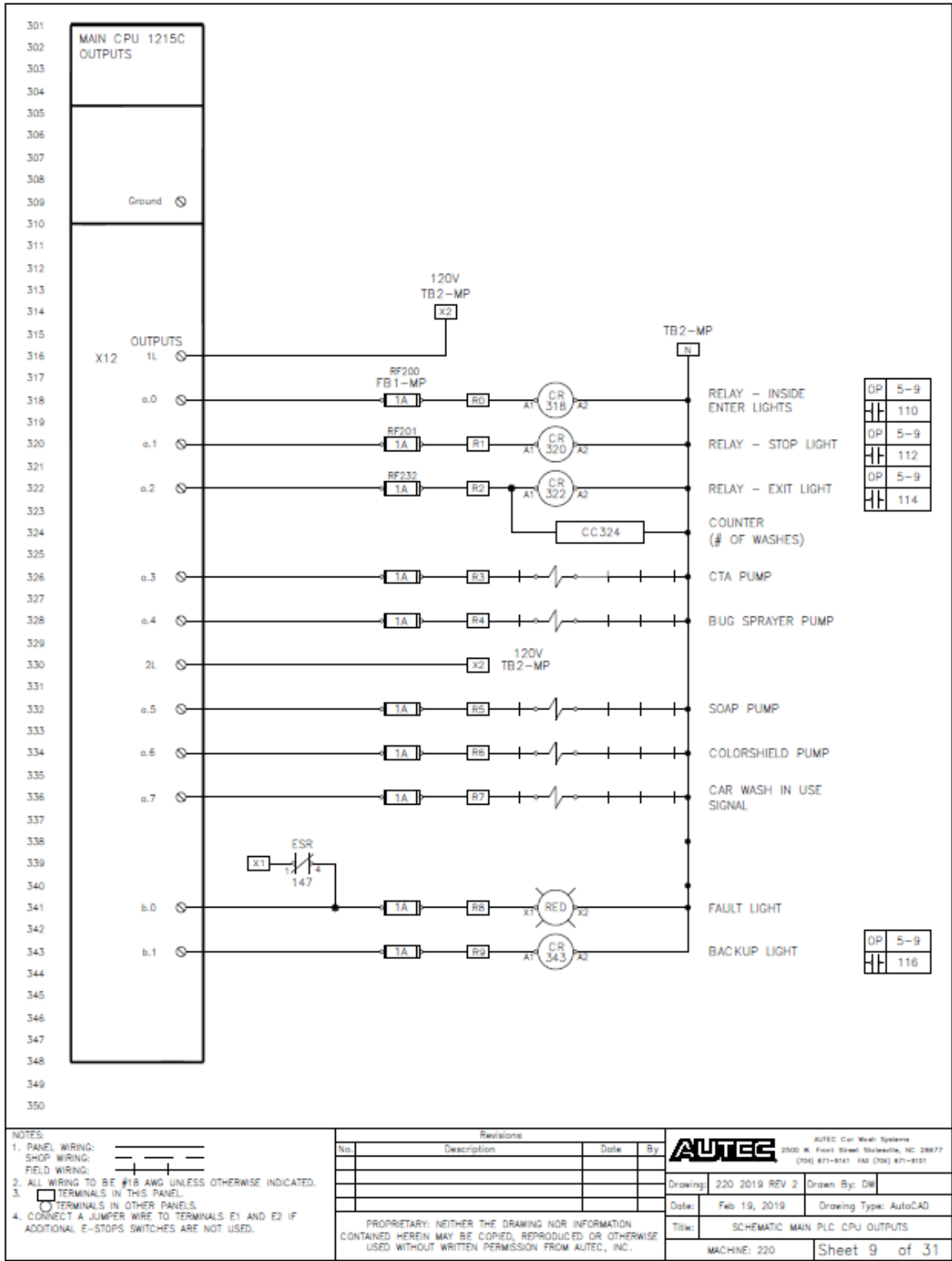
Fig 9-9 Main Control Panel – PLC Main Outputs
