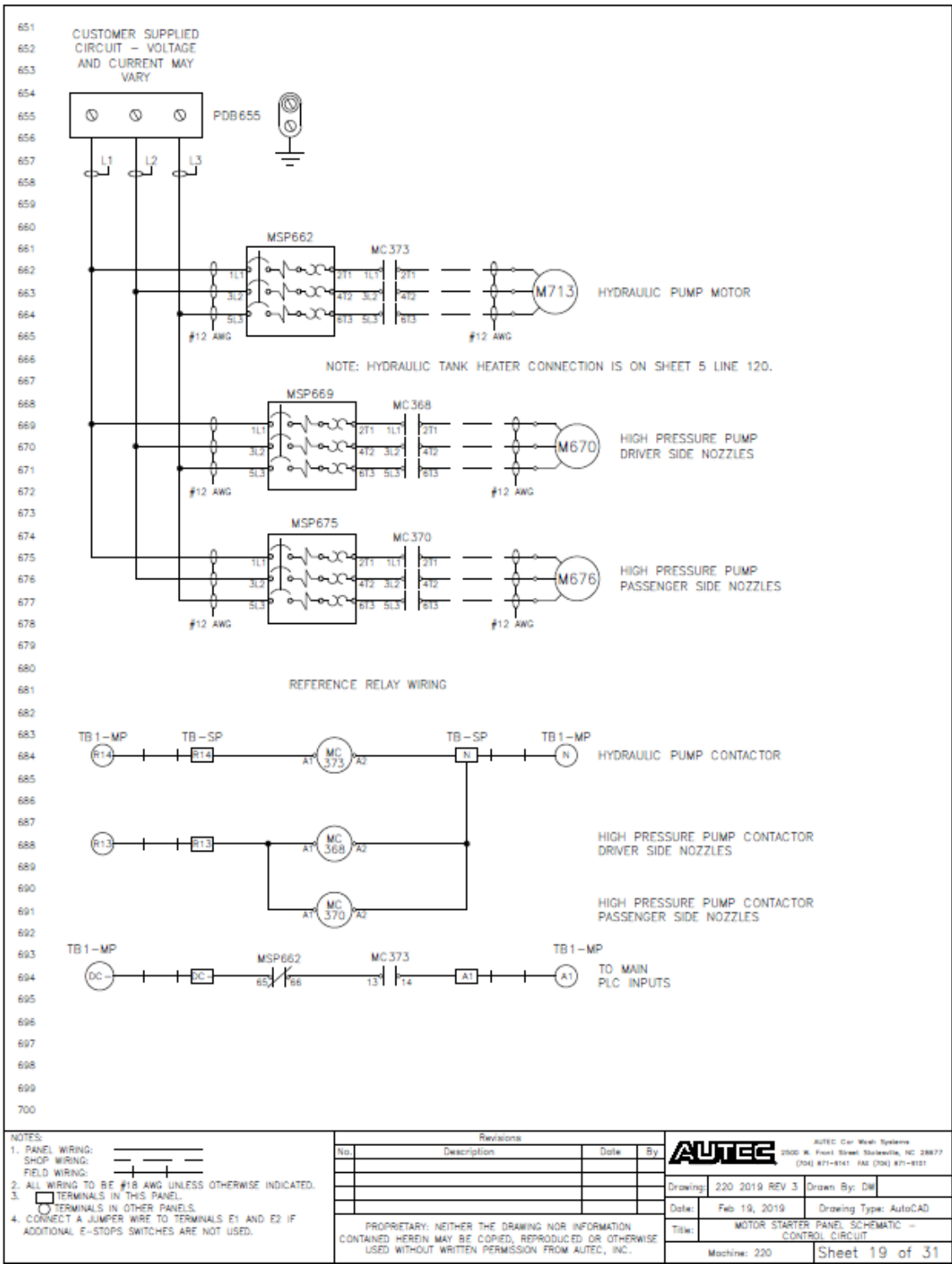
Fig 9-19 Motor Control Panel –Control Circuit
