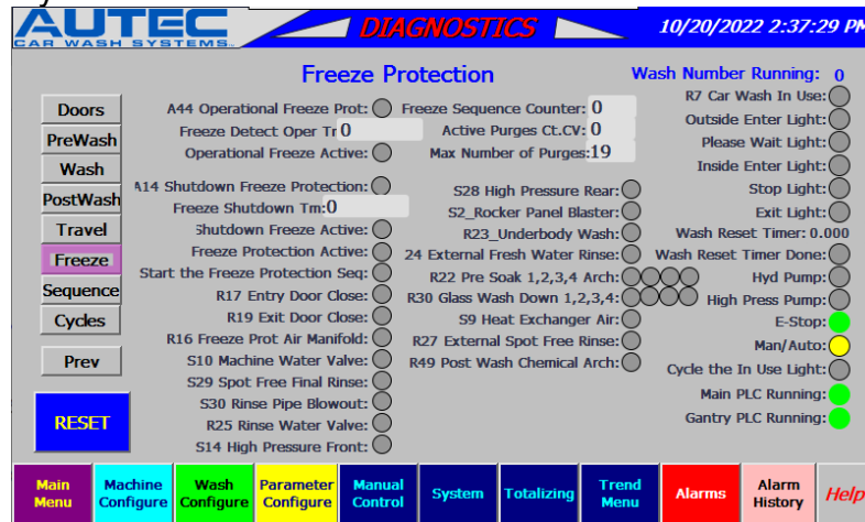
Figure 7-34 Freeze Screen
