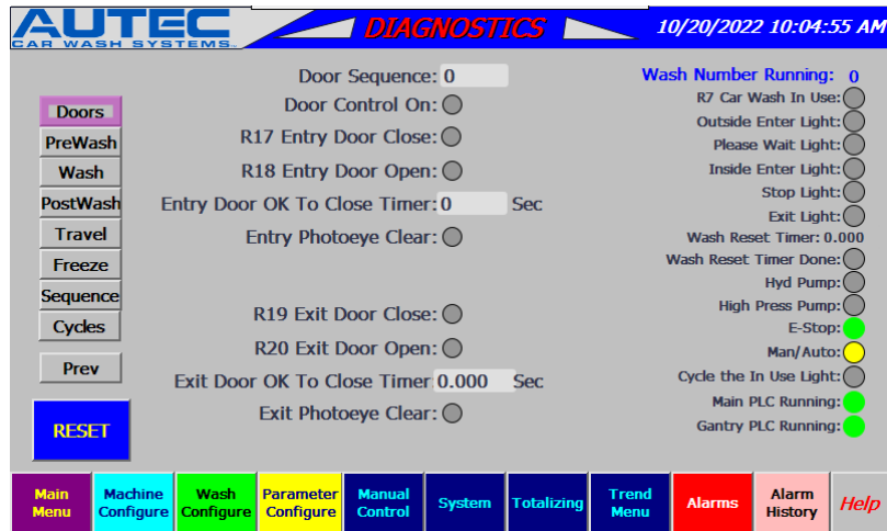
Figure 7-29 Diagnostic Screen - Doors
