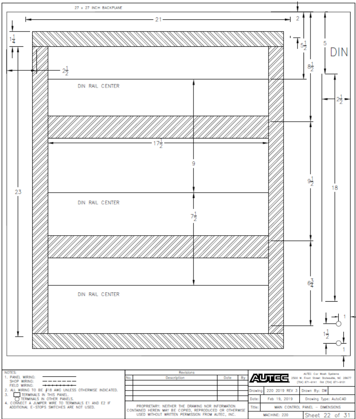
Fig 9-22 Main Control Panel - Dimensions
