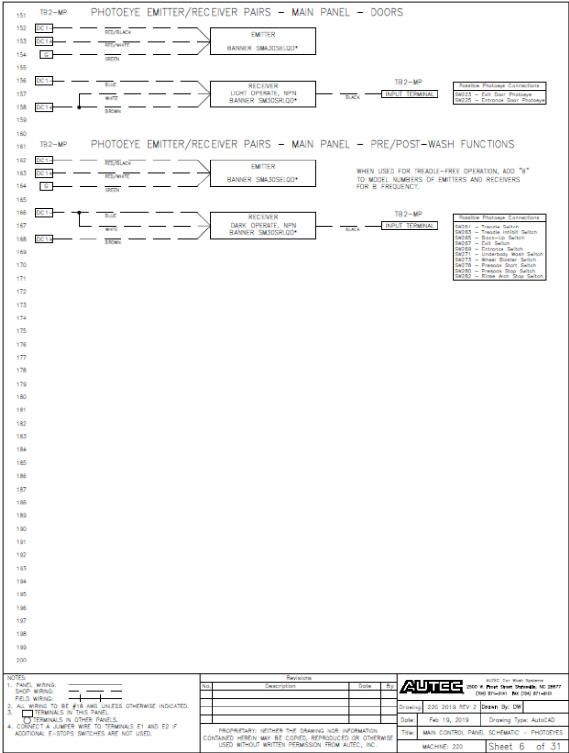
Fig 9-6 Main Control Panel – Photoeyes
