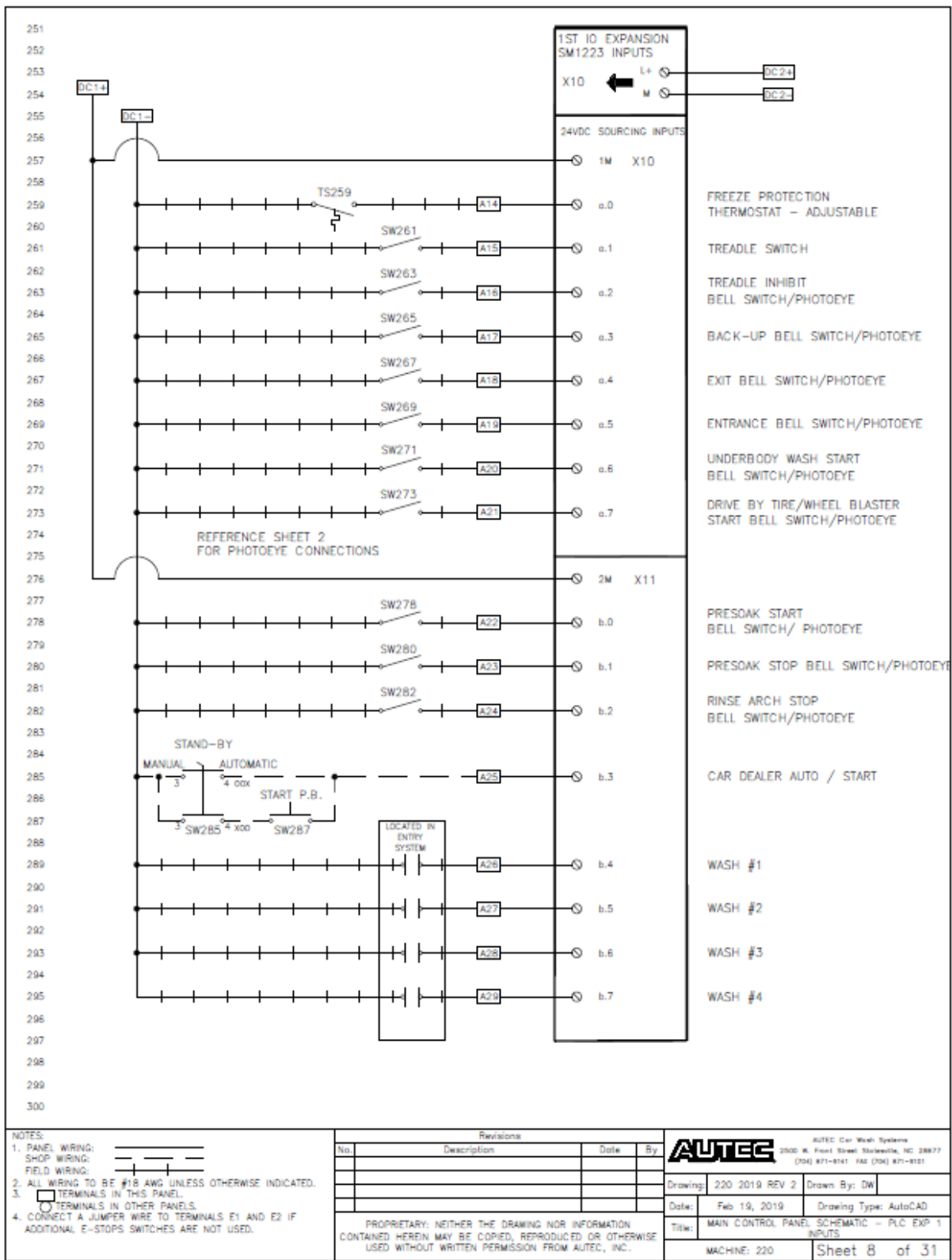
Fig 9-8 Main Control Panel – PLC Module 1 Inputs
