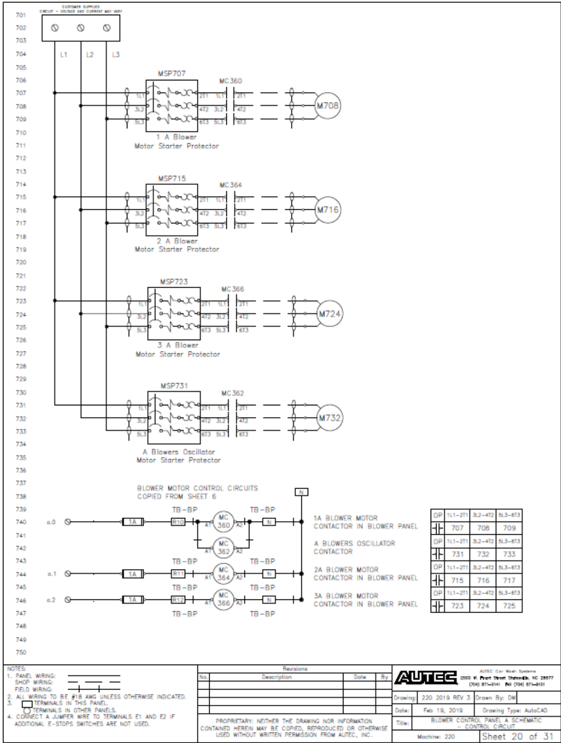
Fig 9-20 Motor Control Panel –Control Circuit
