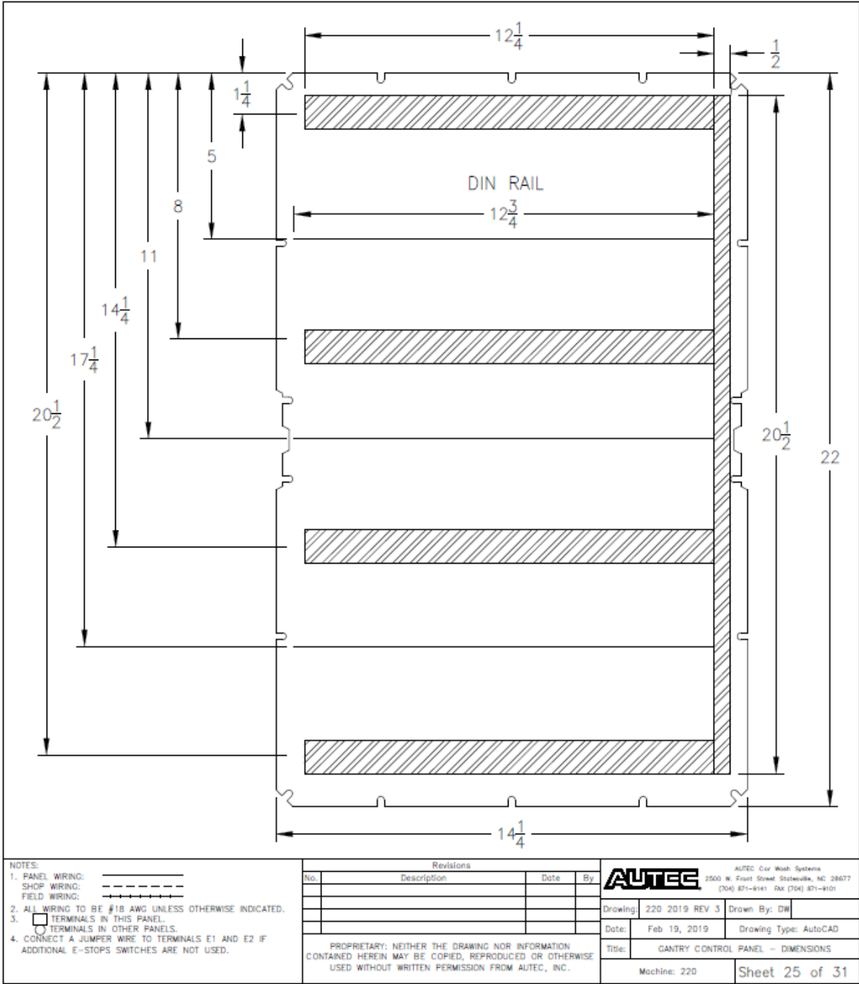
Fig 9-25 Gantry Control Panel - Dimensions
