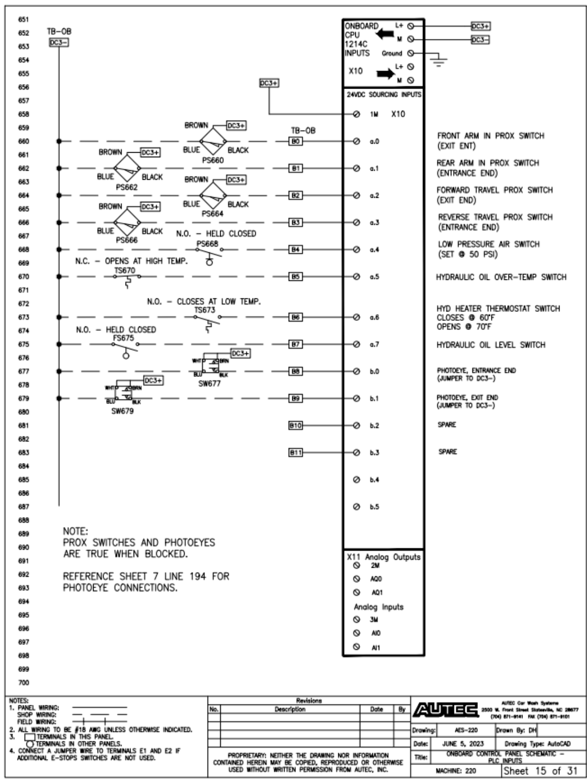
Fig 9-15 Gantry Control Panel – Inputs
