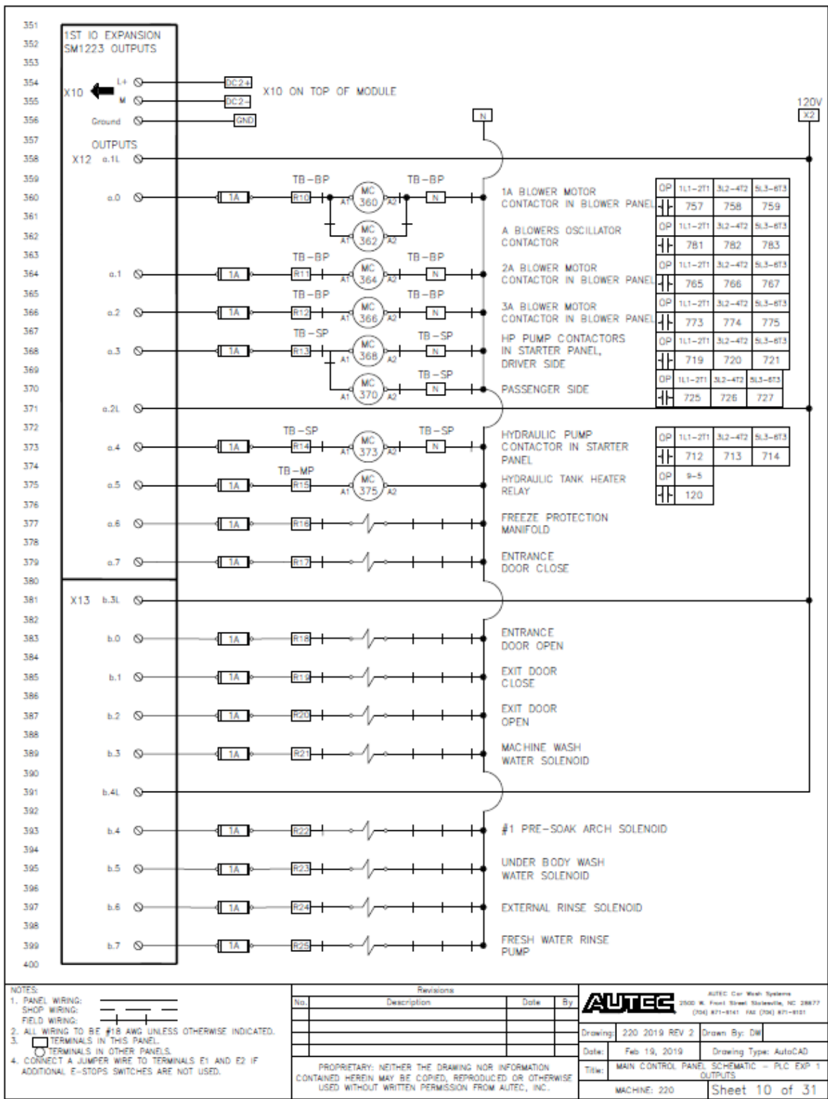
Fig 9-10 Main Control Panel – PLC Module 1 Outputs
