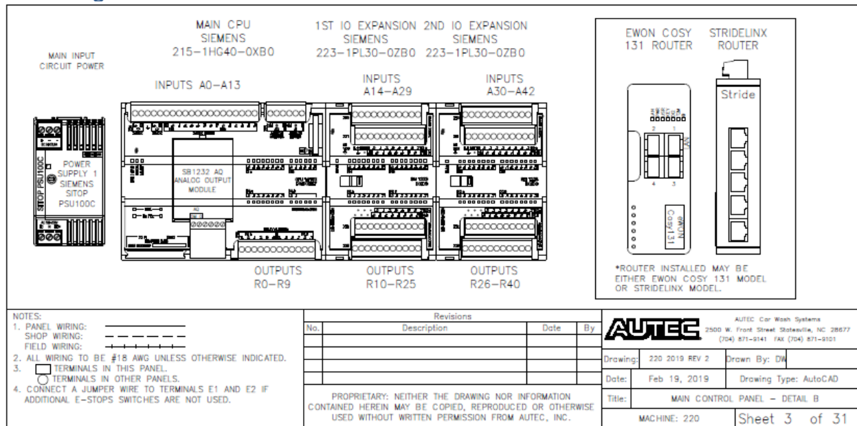
Fig 9-3 Main Control Panel – Detail B
