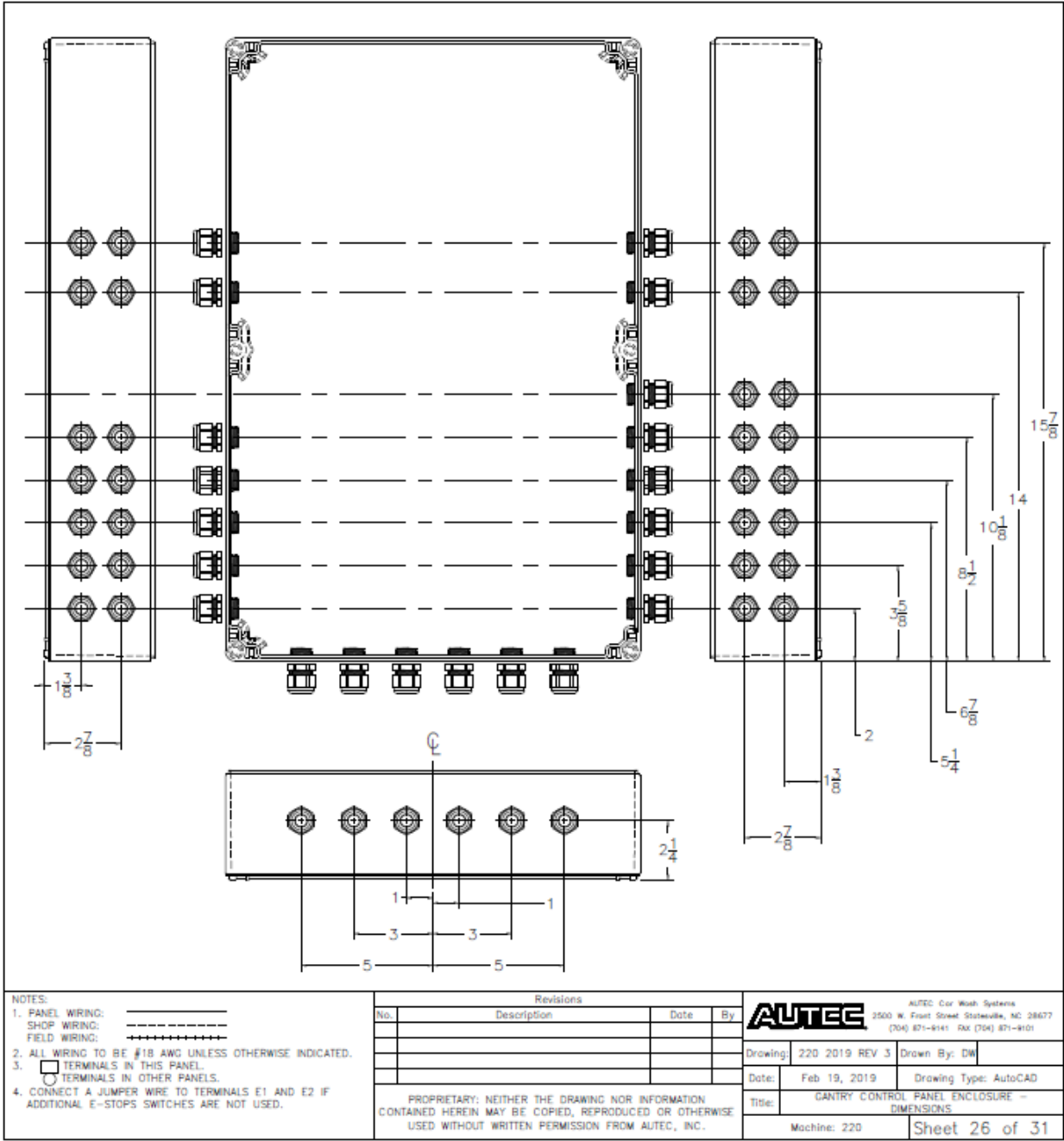
Fig 9-26 Gantry Control Enclosure - Dimensions
