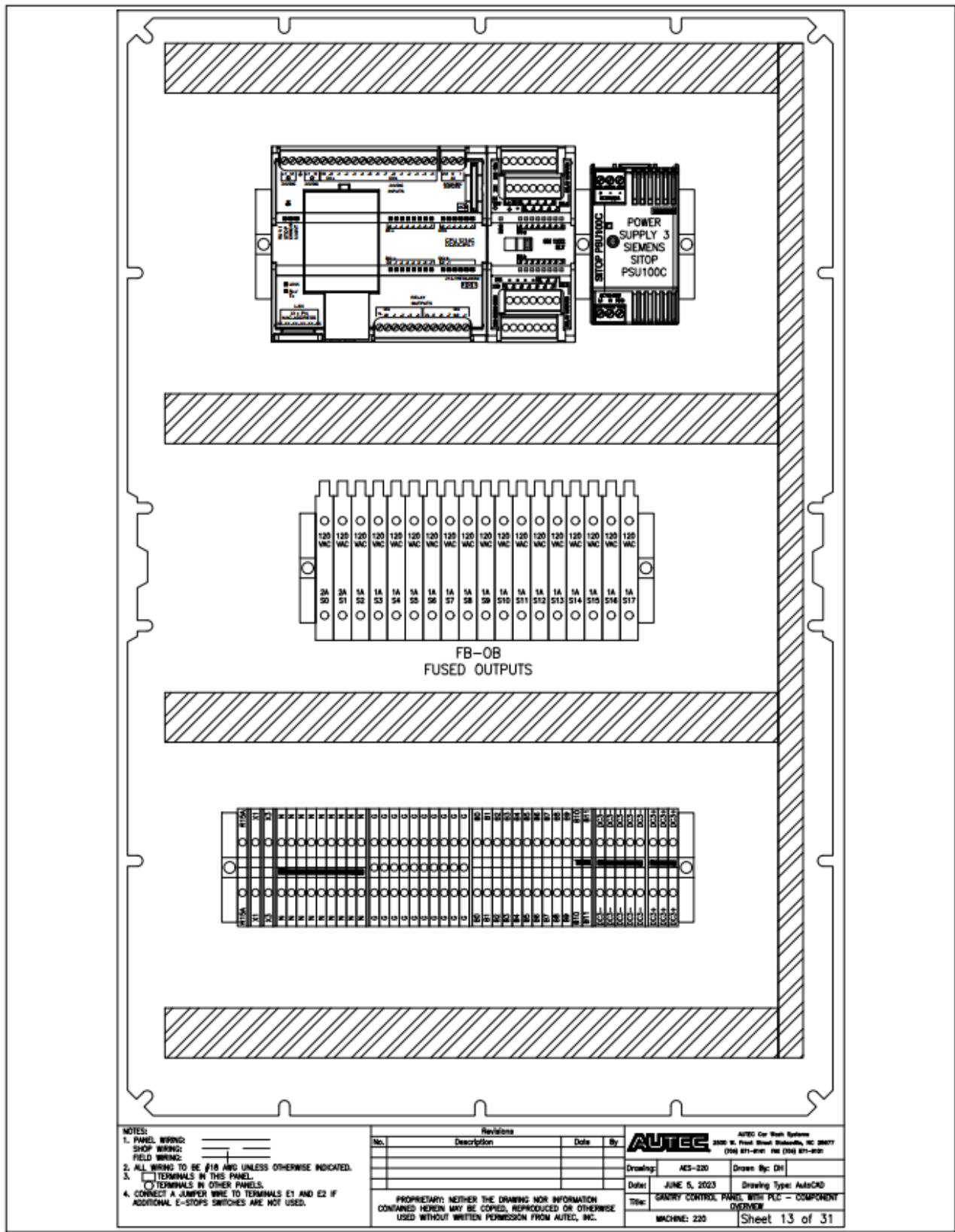
Fig 9-13 Gantry Control Panel – Component Details
