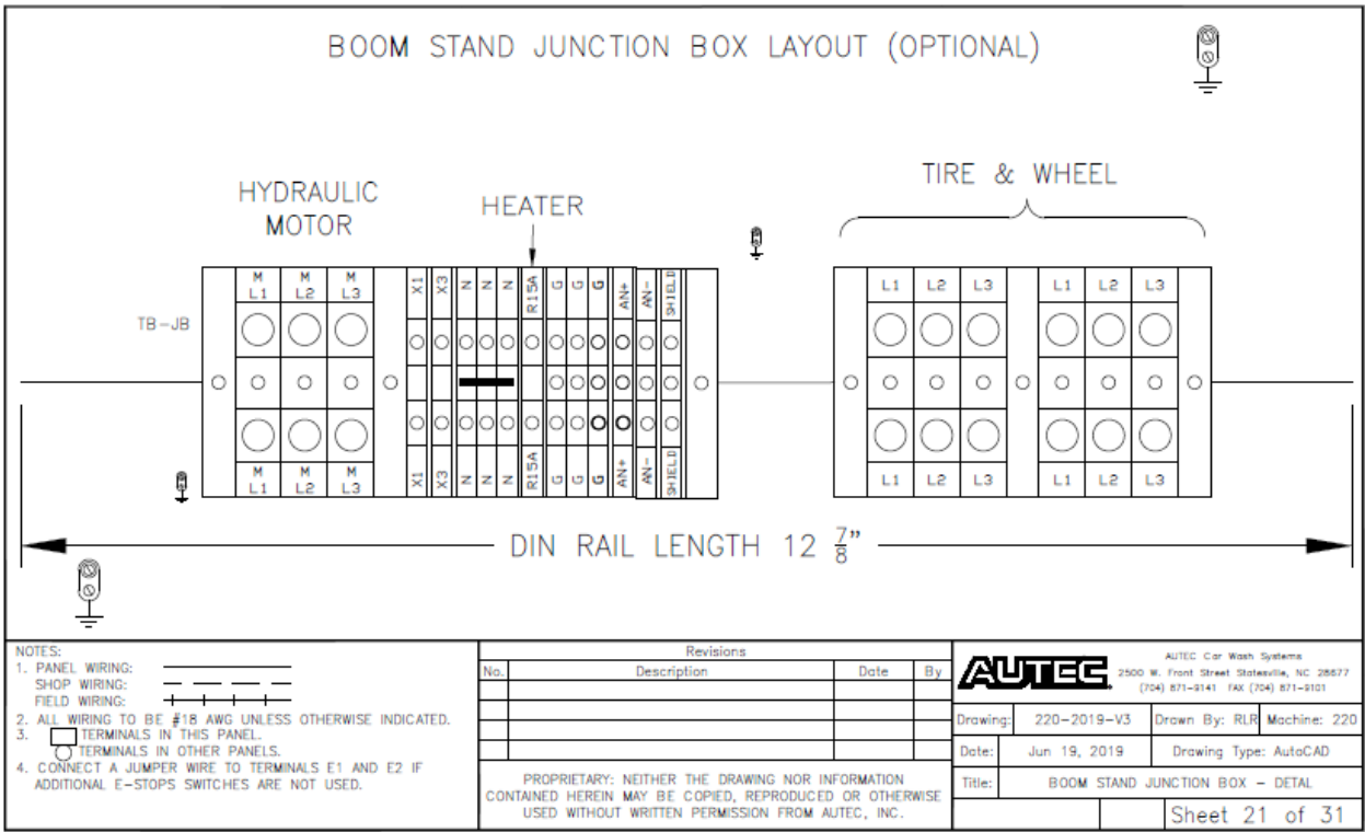
Fig 9-21 Boom Stand Junction Box - Detail
