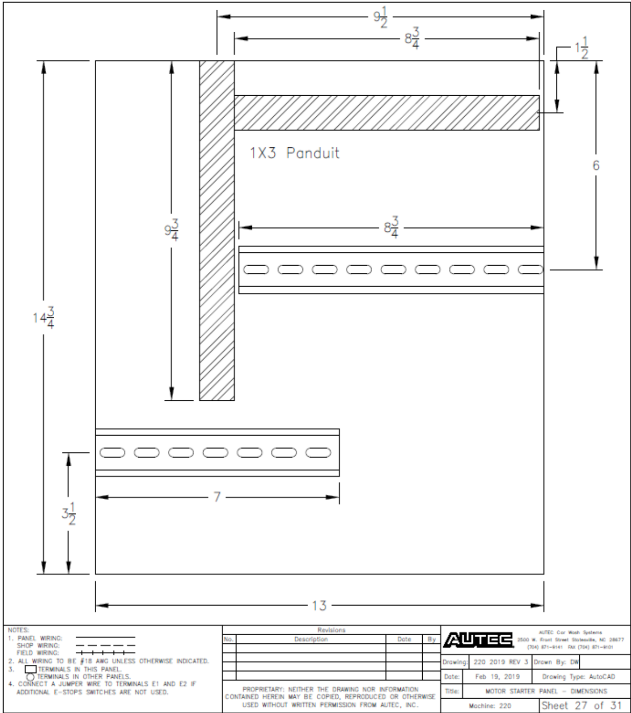
Fig 9-27 Gantry Control Enclosure - Dimensions
